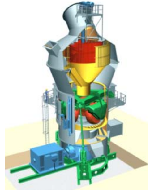
MPS Vertical Roller Mill
